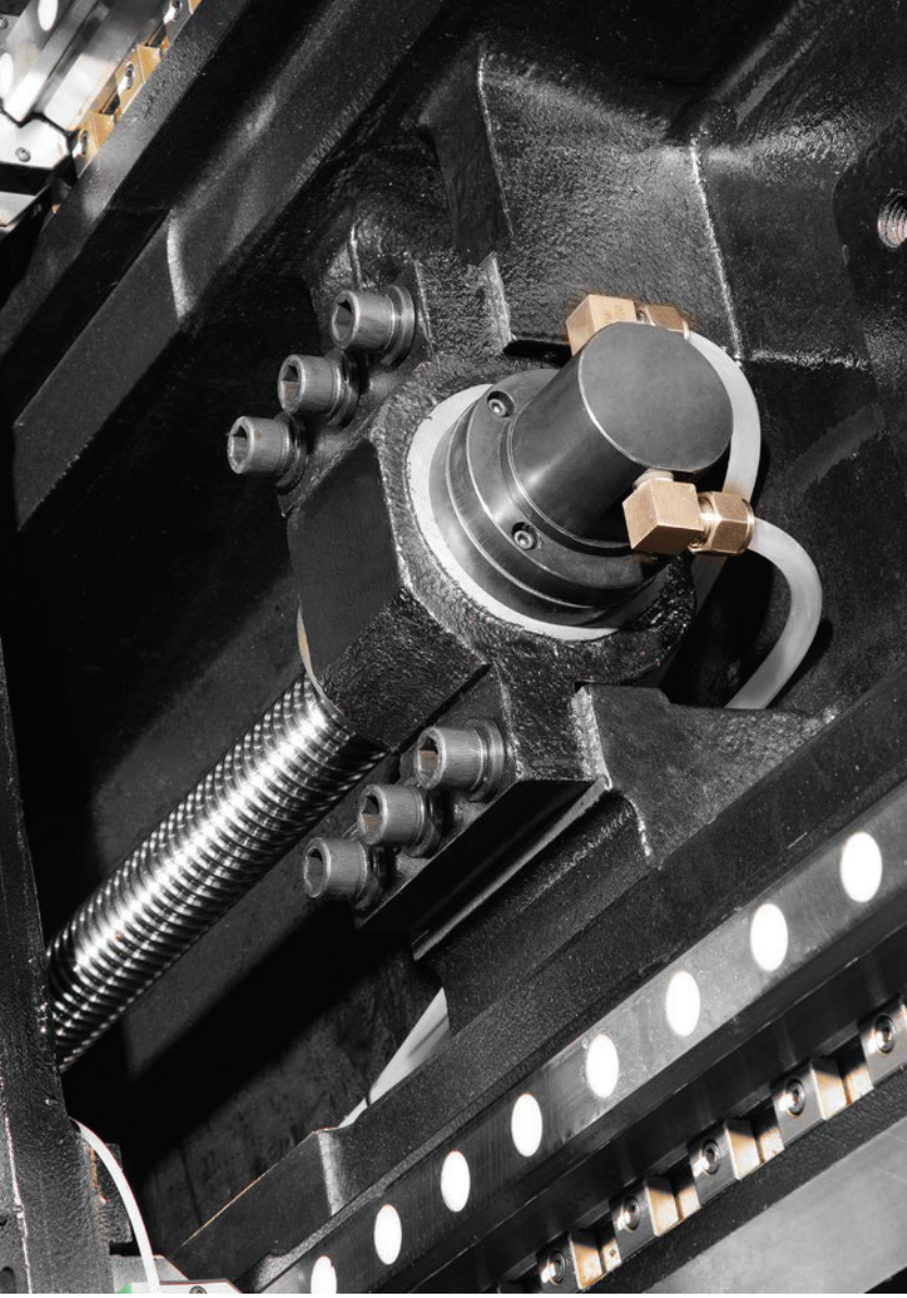
Oil cooling through ballscrew(optional)
